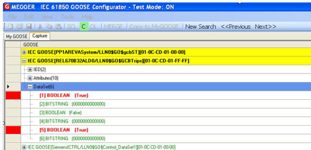
Fig. 9. GOOSE Monitoring, Operation of Protection Function.
