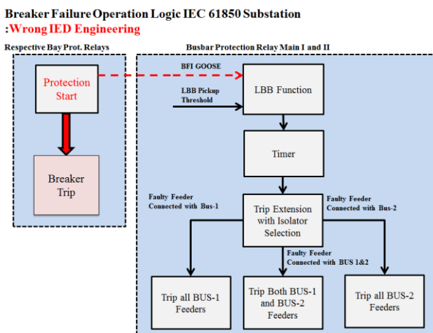
Fig. 5. Breaker Failure Scheme Operation Logic with Improper Configuration.
