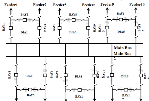
400kV Substation with One and Half Breaker System
